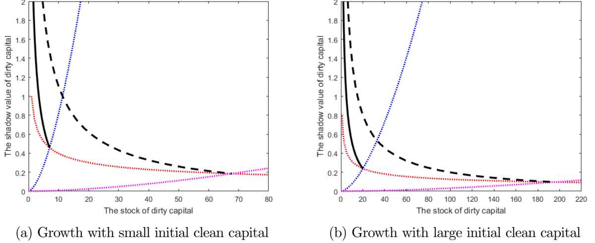
Figure 1: Phase diagrams of growth with direct and indirect irreversibility of investment: (a) growth with smaller initial clean capital endowment K_C^0 = 1 ; (b) growth with larger initial clean capital endowment K_C^0 = 10 . The dotted red, blue and magenta line corresponds to locus of points for stationary dirty capital stock, stationary shadow values with stringent and lax pollution regulations, respectively. The solid and dashed black line corresponds to the stable saddle path of growth with stringent and lax pollution regulations, respectively.
