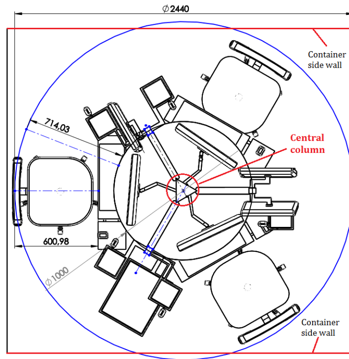
Figure 9. Ground wireframe view of the operators' workstation complex
