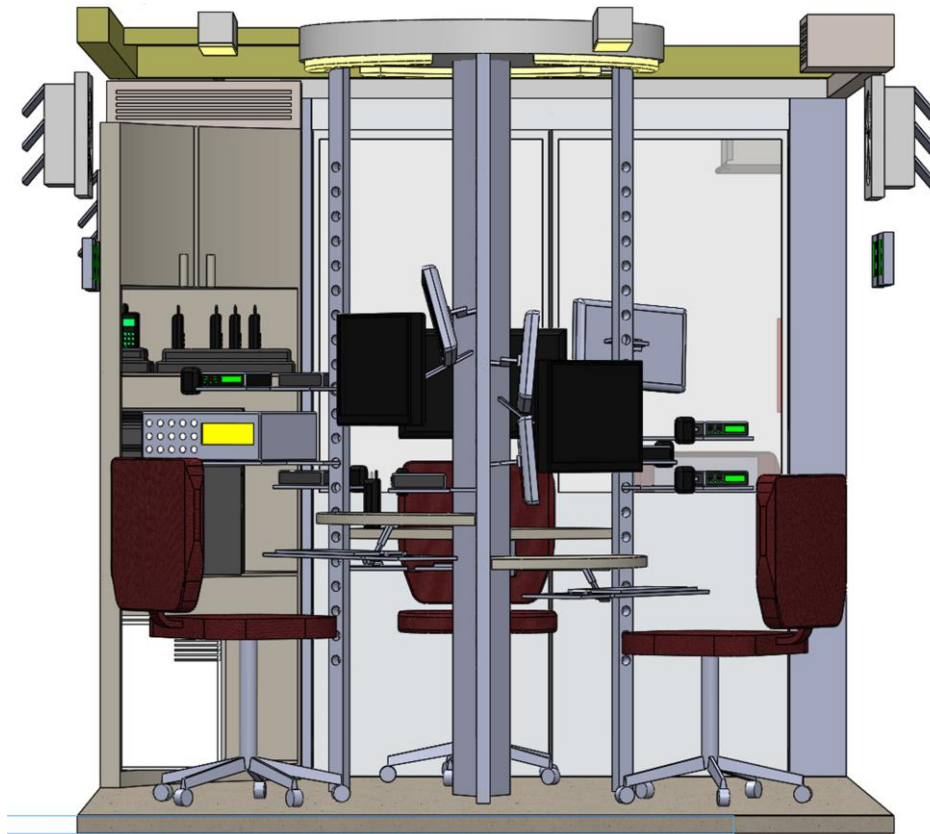
Figure 7. Section view of the operators' area
