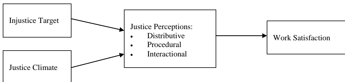
Figure 1: Theoretical Model
