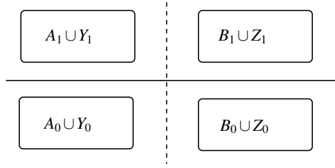
Fig. 10 All edges in (A_1 \cup Y_1) \times (B_0 \cup Z_0) are labeled (-, -) with respect to M^* and all edges labeled (+, +) with respect to M^* are in (A_0 \cup Y_0) \times (B_1 \cup Z_1) .
