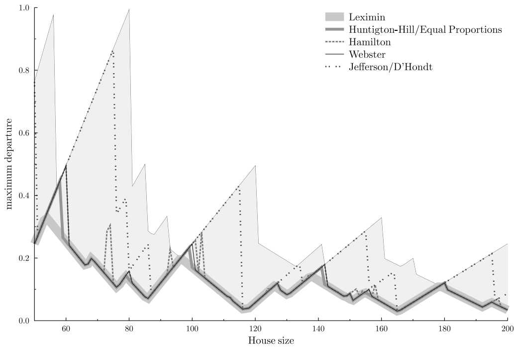
Figure 1: Apportionment over Belgian regions. Leximin coincides with \beta ; EP, Webster are near. Ironically D'Hondt performs poorly reaching \omega several times.
