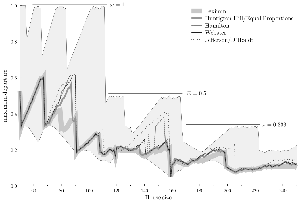
Figure 2: Apportionment over Irish counties. Leximin performs best, then EP, Webster, but all struggle to evenly distribute seats due to regular county sizes.
