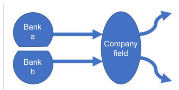
Figure 2: Ability-to-nurture Paradigm
