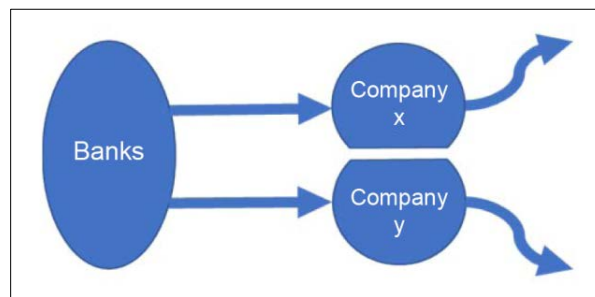
Figure 1: Ability-to-pick Paradigm
