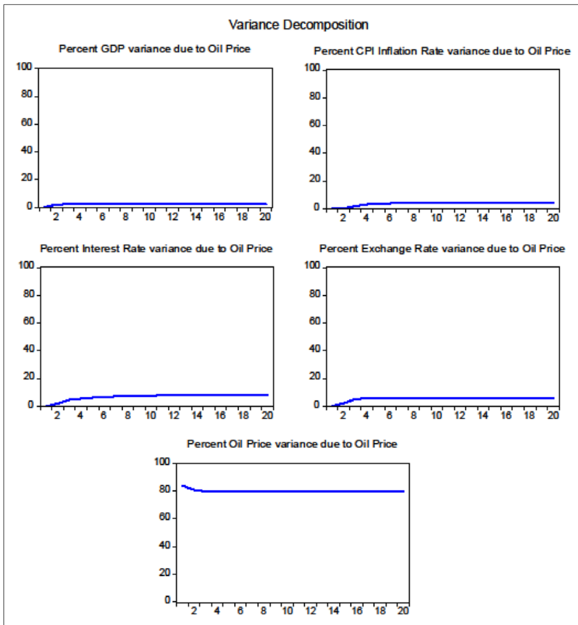
Figure 8: Variance Decomposition
