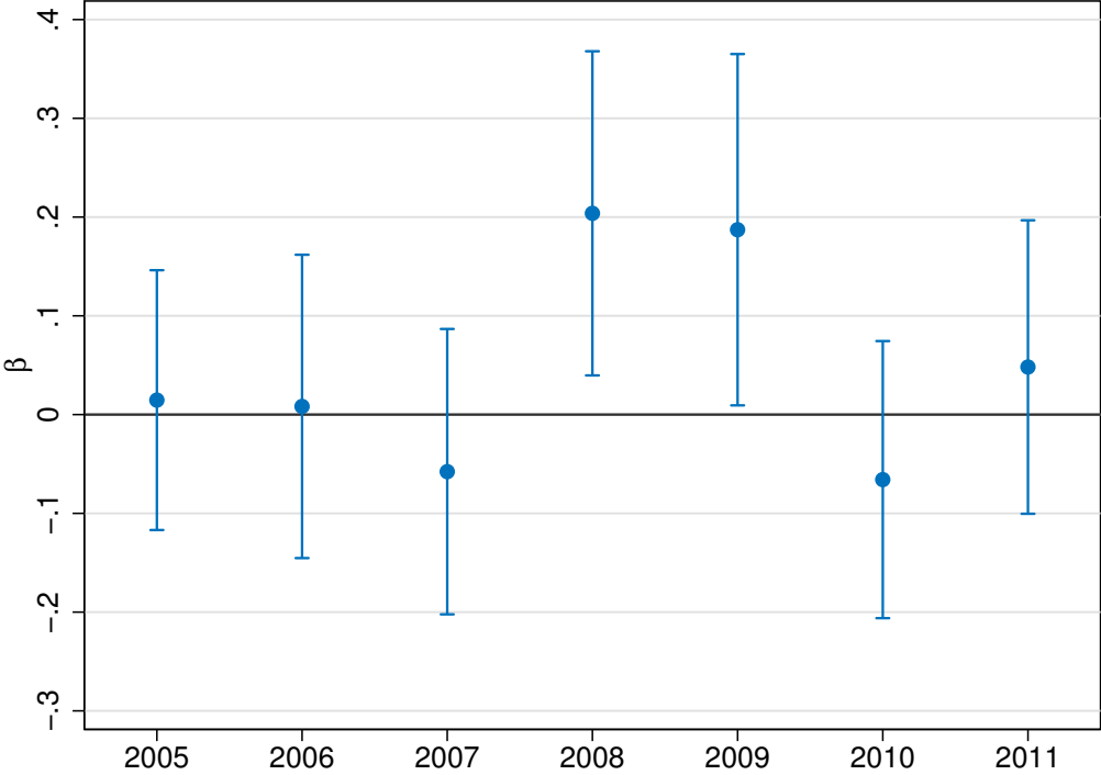
Figure 2: Pre-Treatment Trends
