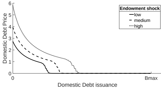
(a) Domestic debt price conditional on no external debt issued
