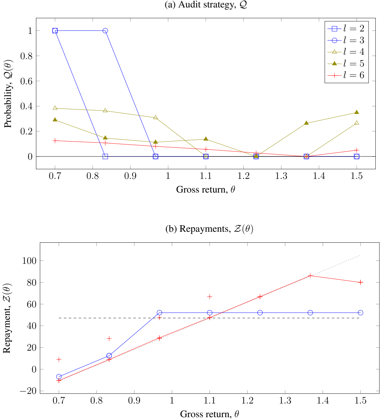
Figure 3: Numerical example
