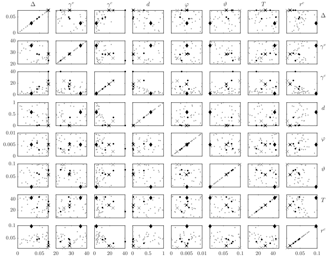
Figure 5: euro area, |\mathcal{M}_{90}| = 34 , |\mathcal{K}| = 6 , ♦ = 364
