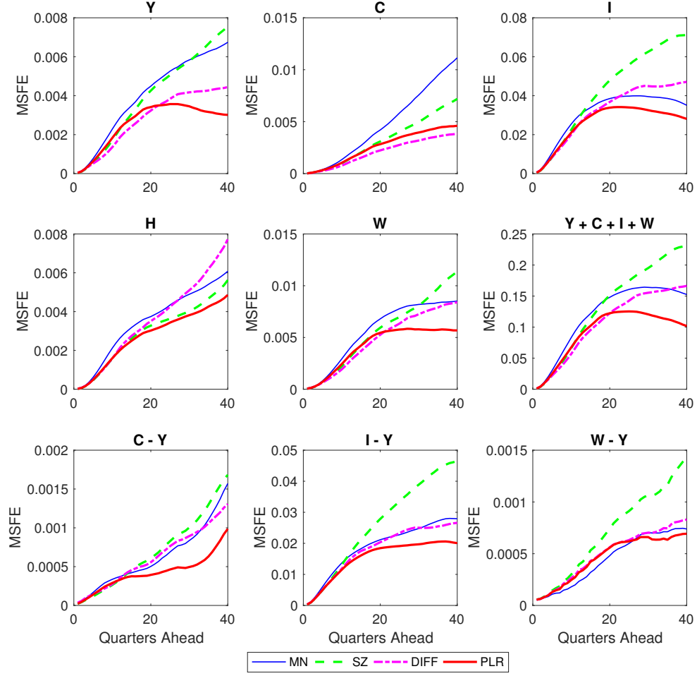
FIGURE 3.1. Mean squared forecast errors in models with five variables. MN: BVAR with the Minnesota prior; SZ: BVAR with the Minnesota and sum-of-coefficients priors; DIFF: VAR with variables in first differences; PLR: BVAR with the Minnesota prior and the prior for the long run.
