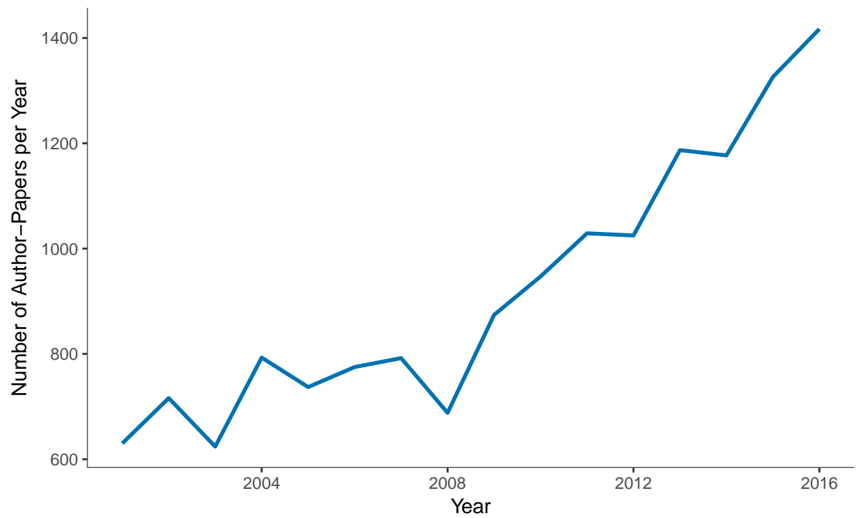
Figure A4: Number of Paper-Authors over Time
