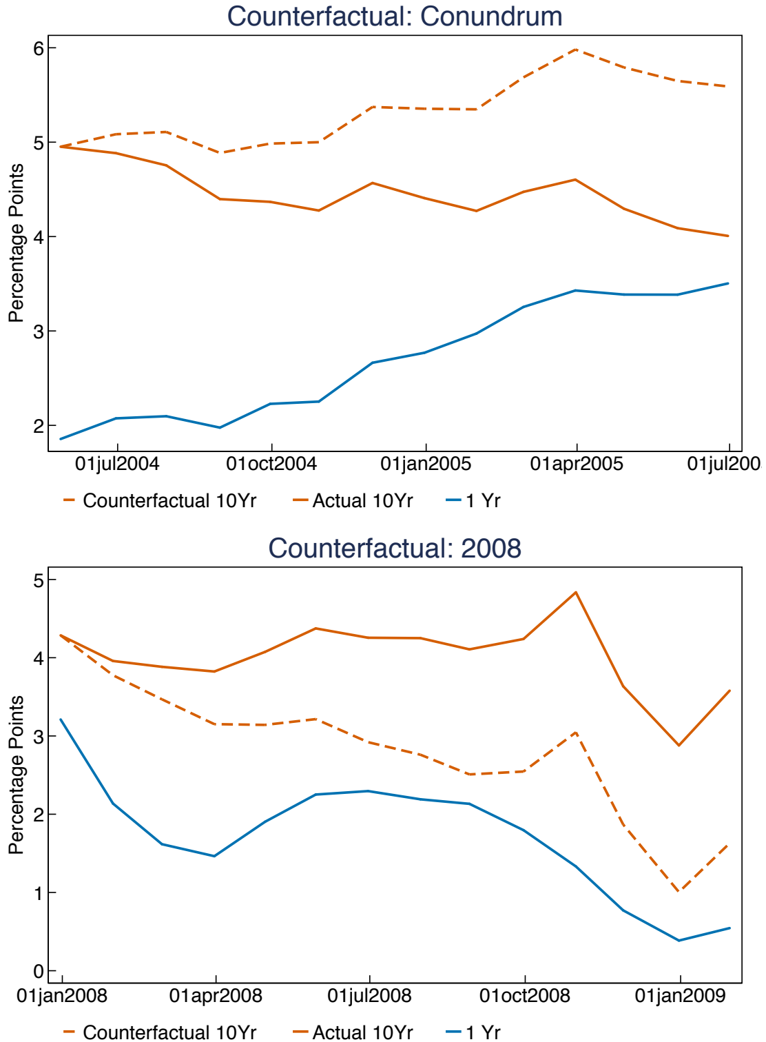
Figure 4: Counterfactual paths of ten-year yields in selected episodes This figure plots one- and ten-year yields in the original “conundrum” period and in 2008, along with counterfactual ten-year yields generated from restricting the slope to depend on lags of level and slope, but not also on lagged changes, as described in the text.
