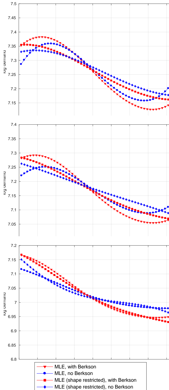
Figure 5: MLE estimates across the income distribution (at \tau = 0.50 )
