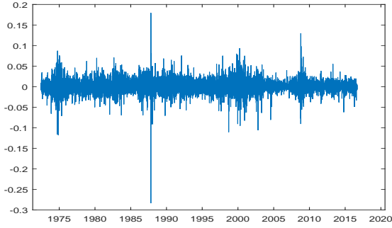
(a) Daily return of Coke
