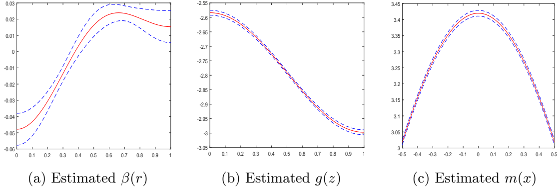
Figure 6: Plot of estimated functions and confidence curves at 95% level
