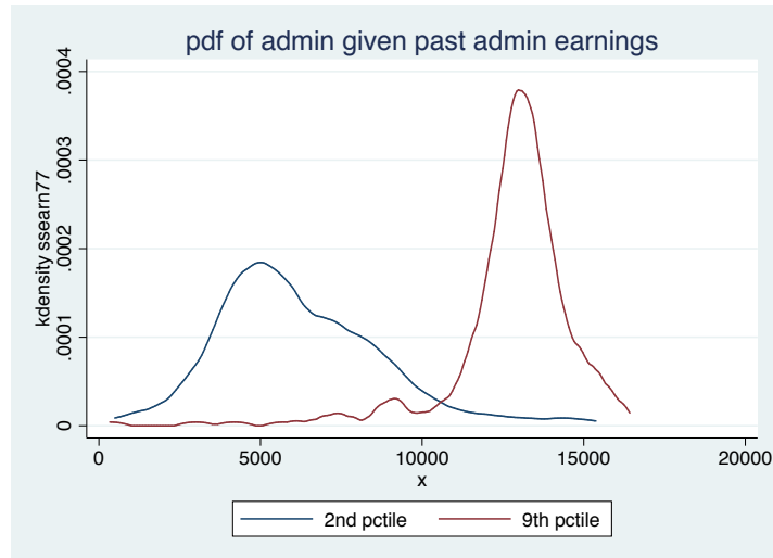
Figure 3: Nonparametric estimate of the conditional density of administrative earnings in 1977 given lagged administrative earnings being in the 2nd or 9th percentile. Bandwidths are chosen by cross-validation.
