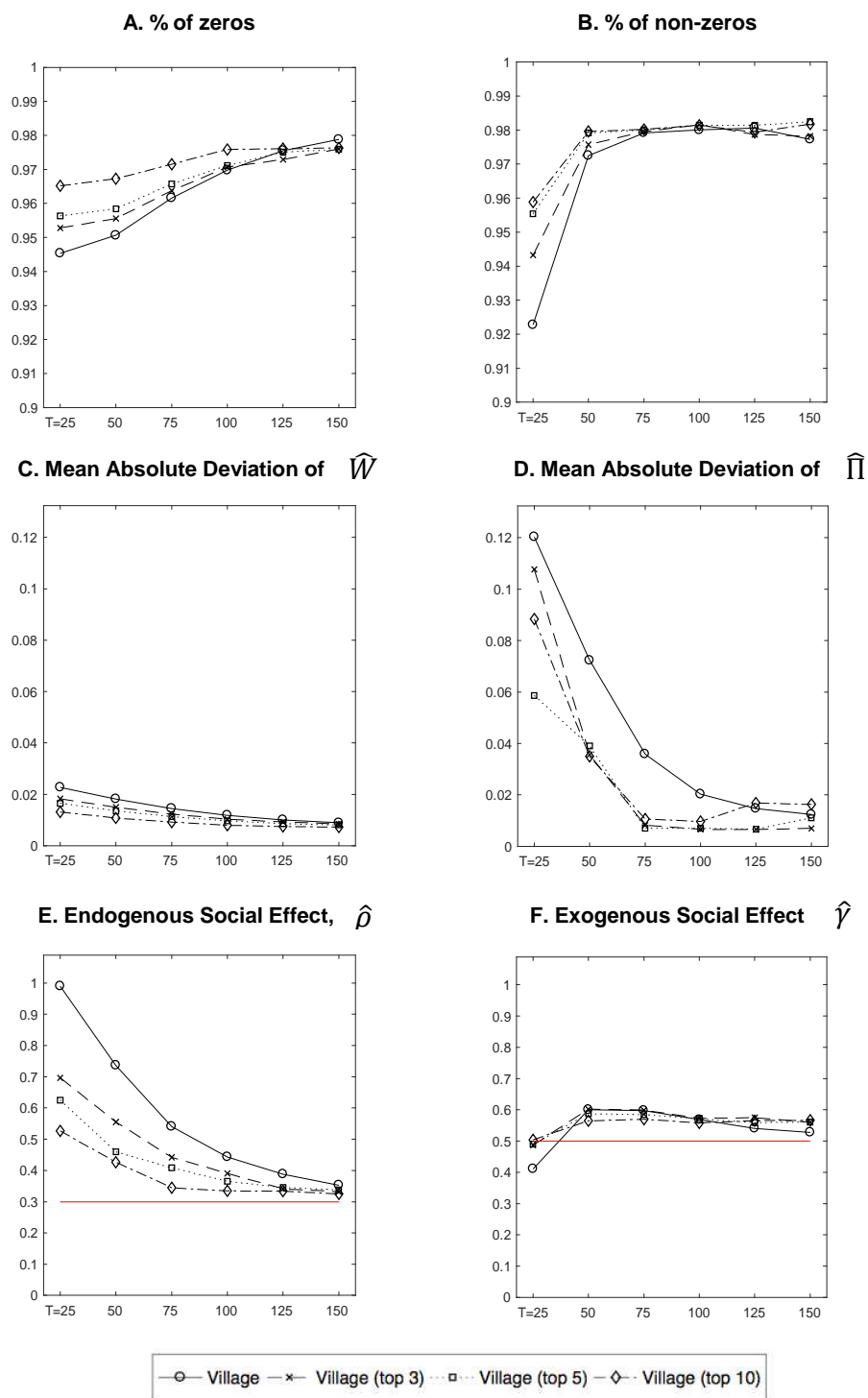
Figure A1: Simulation Results, Adaptive Elastic Net GMM Partial Knowledge of W_0
