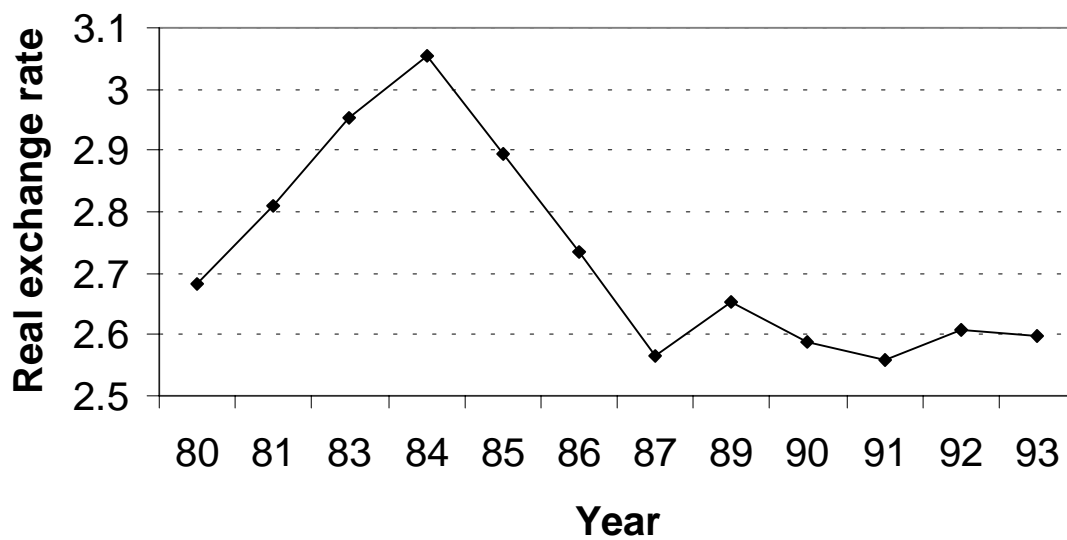
Figure 5: Transport Equipment, SIC 37
