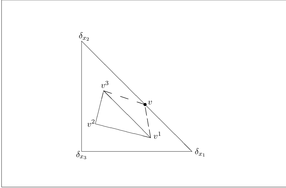
Figure 7: Illustration for Lemma 10
