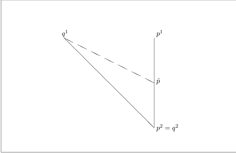
Figure 6: Illustration for Lemma 9
