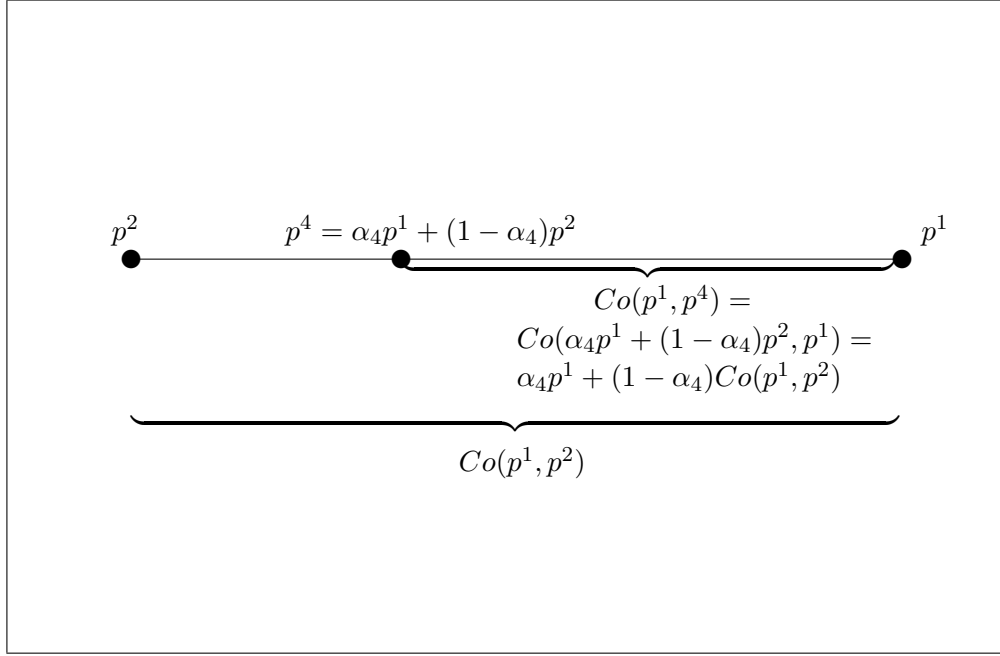
Figure 4: Illustration for Lemma 7
