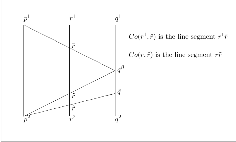
Figure 5: Illustration for Lemma 8
