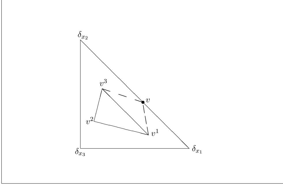
Figure 7: Illustration for Lemma 10
