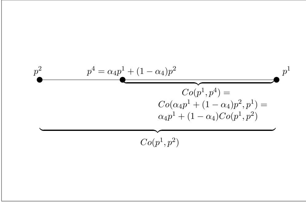
Figure 4: Illustration for Lemma 7
