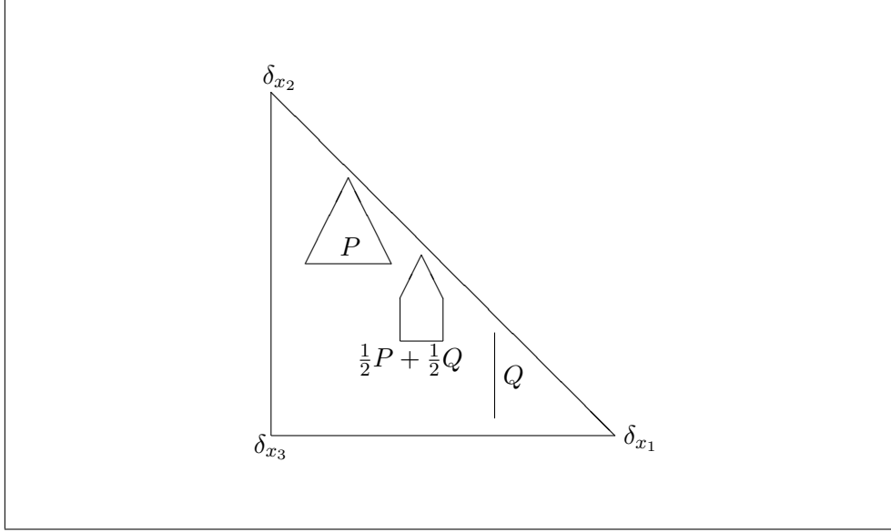
Figure 2: Convex combination of a triangular set P and a line segment Q
