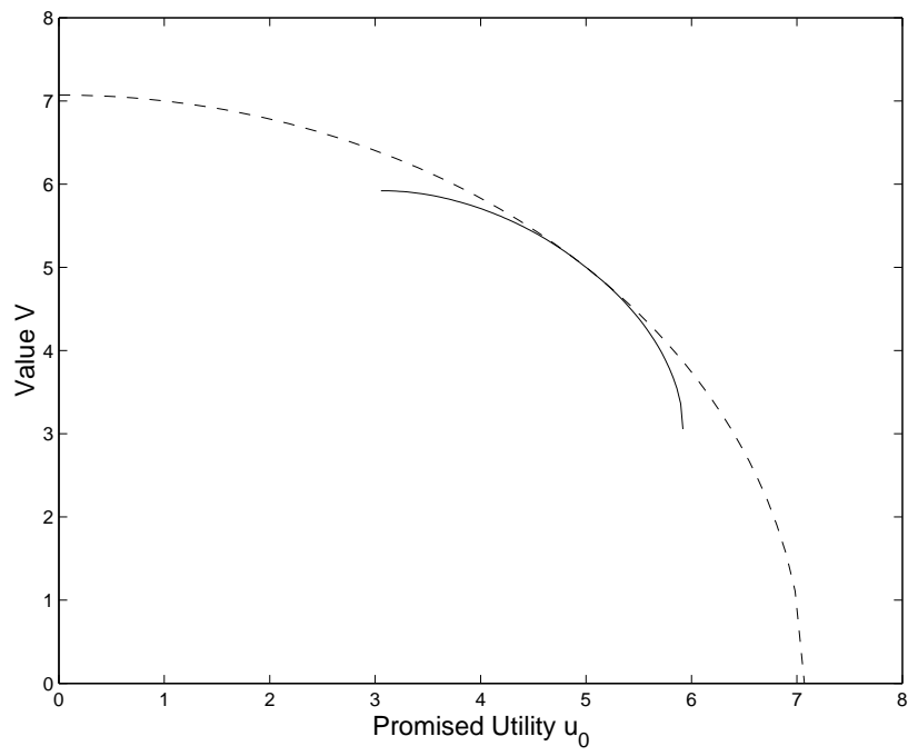
Figure 1: Value Function
