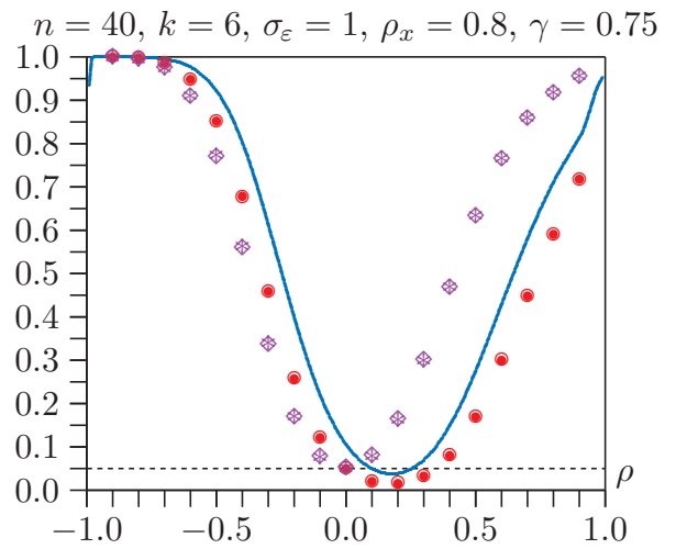
Figure 6. Power of Durbin-Godfrey tests at .05 level
