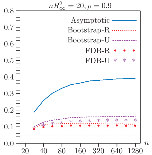
Figure 11. Rejection frequencies for 2SLS t tests at .05 level
