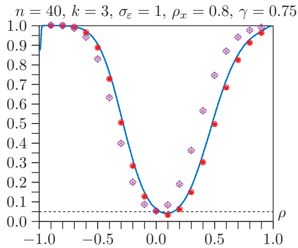
Figure 3. Power of Durbin-Godfrey tests at .05 level
