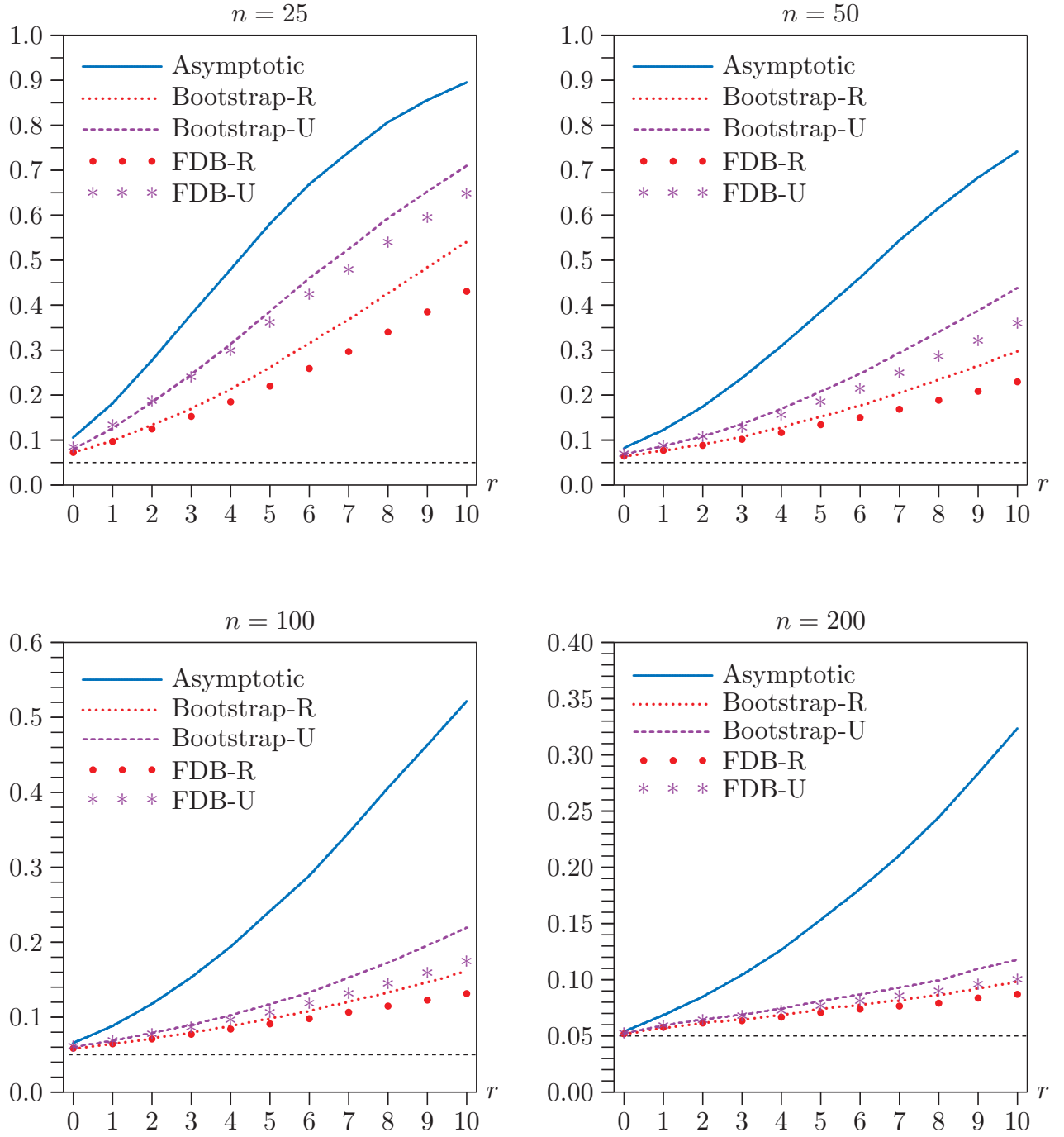
Figure 8. Rejection frequencies for 2SLS t tests at .05 level, R_{\infty}^2 = 0.2 , \rho = 0.9
