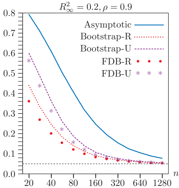
Figure 11. Rejection frequencies for 2SLS t tests at .05 level
