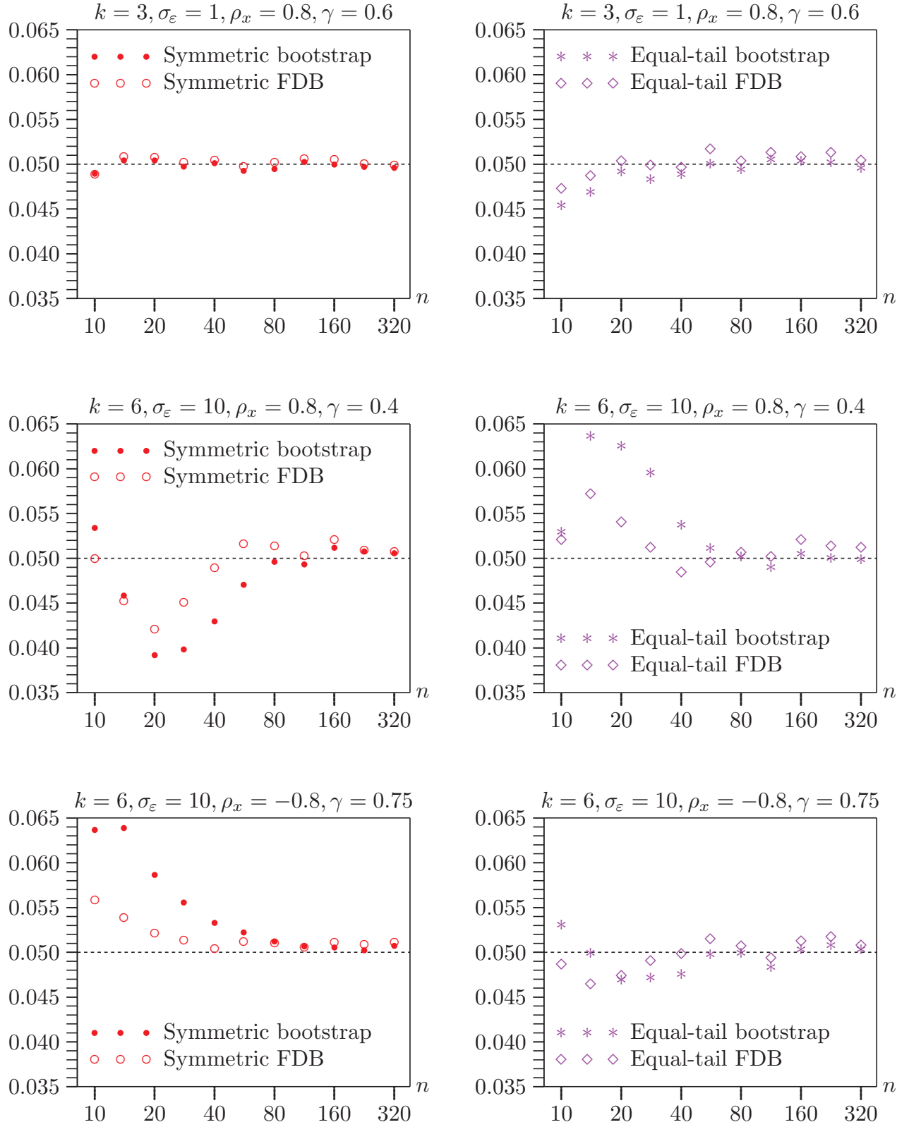
Figure 2. Durbin-Godfrey test rejection frequencies at .05 level under the null
