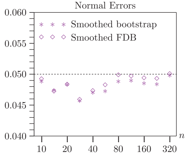
Figure 4. ARCH test rejection frequencies at .05 level under the null
