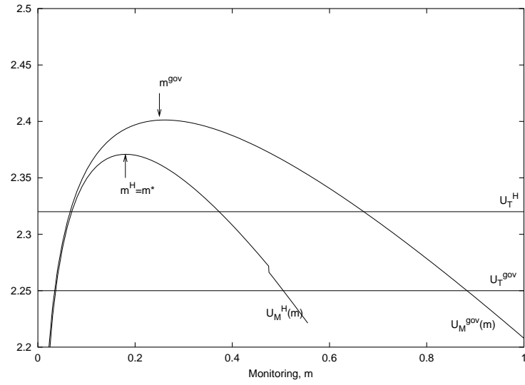
Figure 3: Example 4, High types in the majority.
