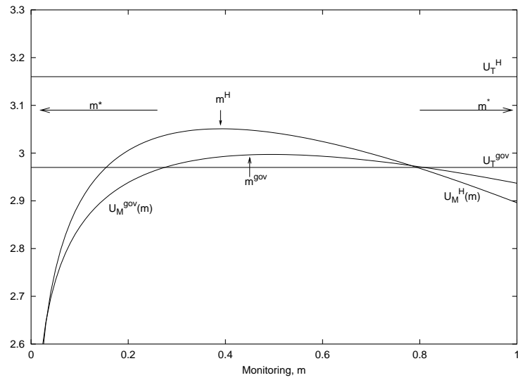
Figure 4: Example 5, High types in the majority.
