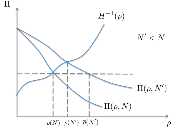
Figure C.1: Counterfactual bounds
