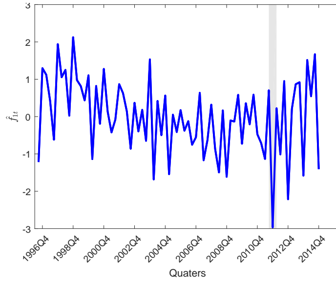
Figure 3: Developed economy activity factor
