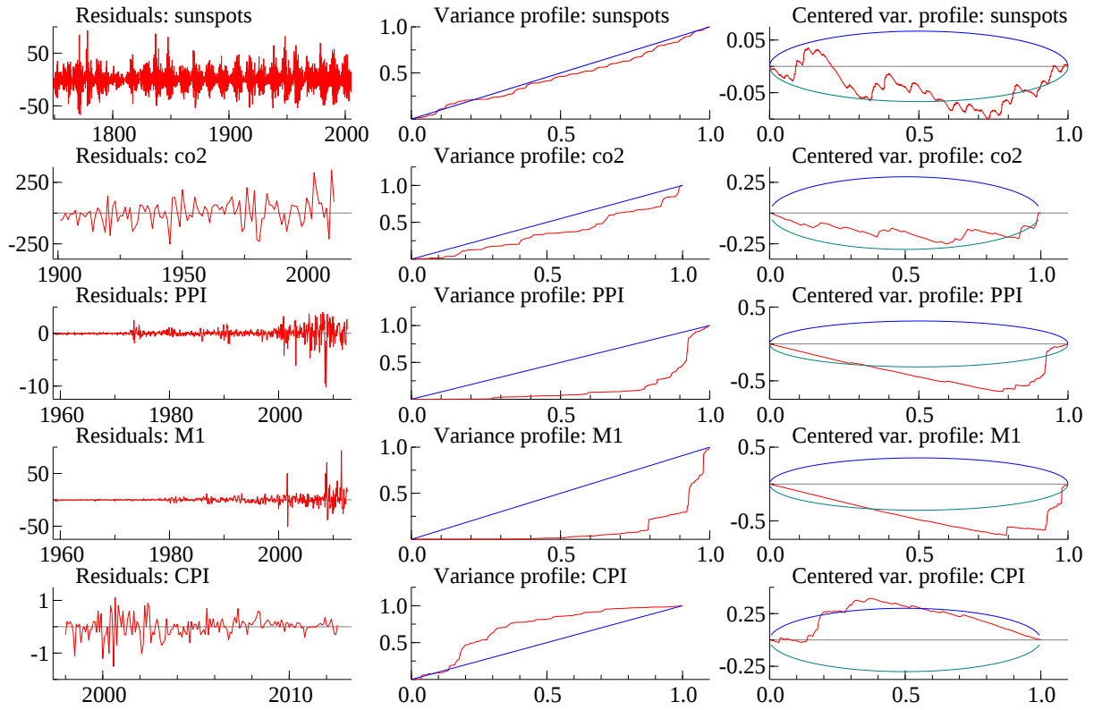
Figure C.1: Residual graphics for data examples
