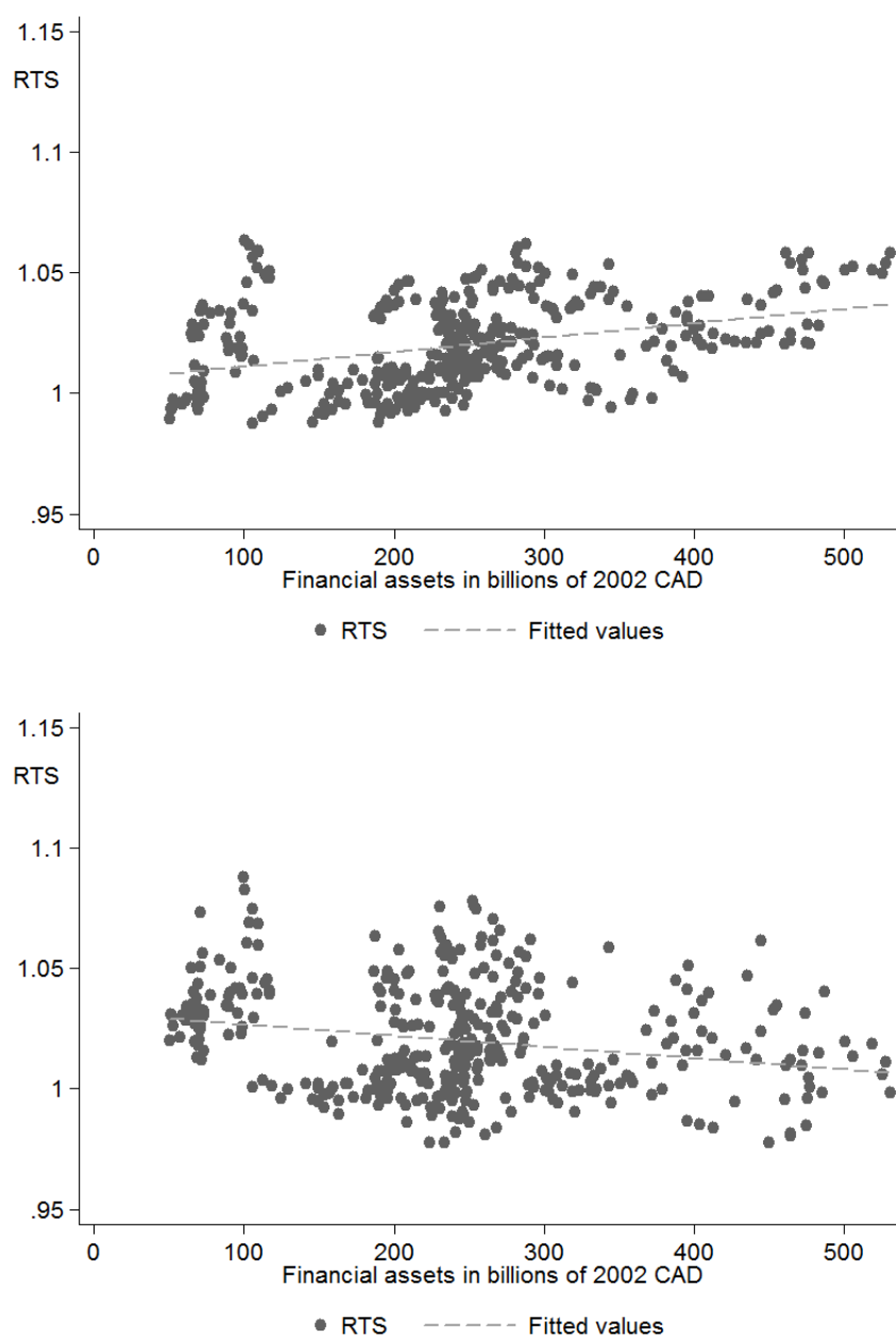
Figure 19: Long-run RTS
