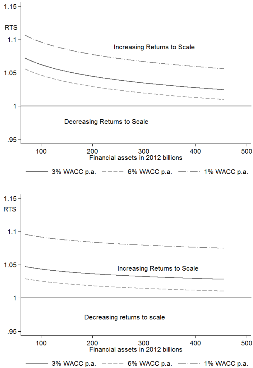
Figure 18: Long-run RTS
