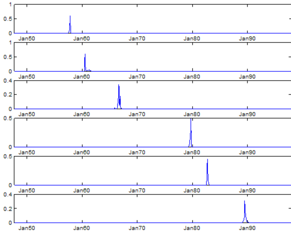
Figure 2: Posterior probability of break occurrence for the AR(1) model, assuming K = 6 breaks.
