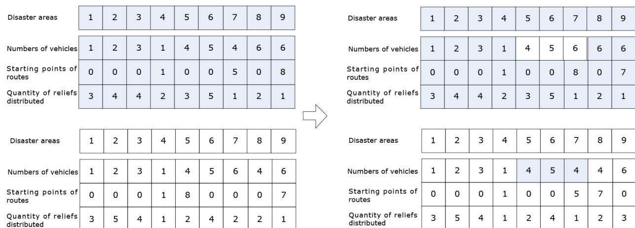
Figure 5. Diagram of the two-point crossover operation
