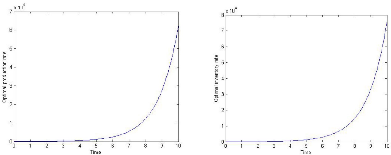
Figure 2. Optimal production rate and optimal inventory rate for parameters
