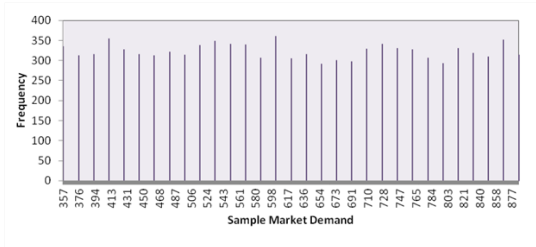
Figure 3. Histogram of a sample market demand when \beta = .1
