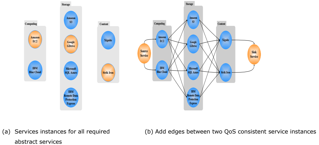
Figure 3. Illustration of on-demand finance service
