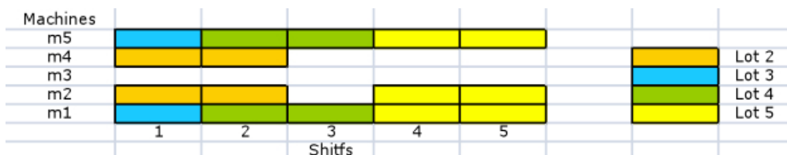
Figure 5. "Solution obtained by scheduling model for instance number 5". Source: Authors
