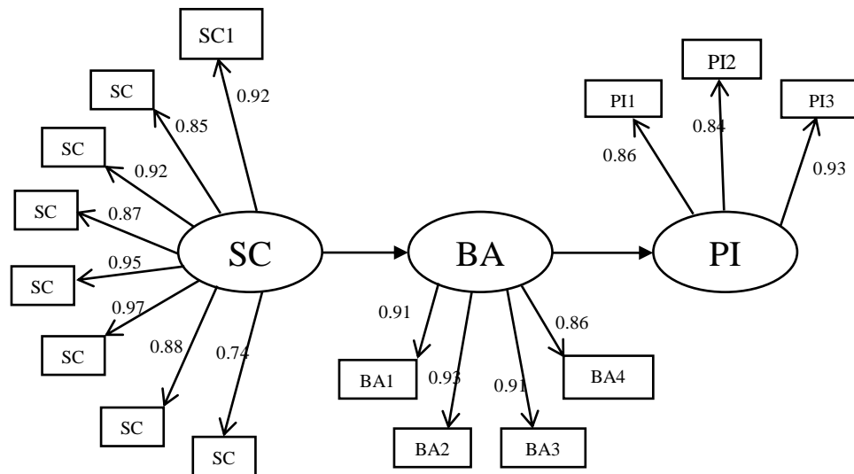
Figure 2: Measurement Model
