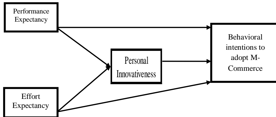
Figure 1: Study Model
