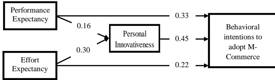
Figure 2: Path analysis
