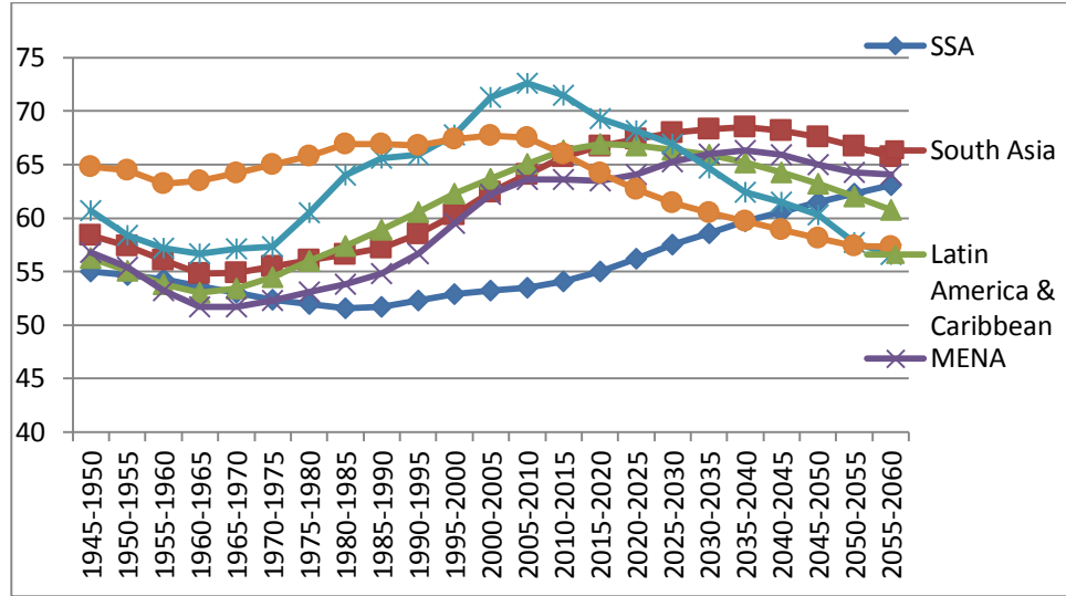
Figure 1: Working-Age Population
