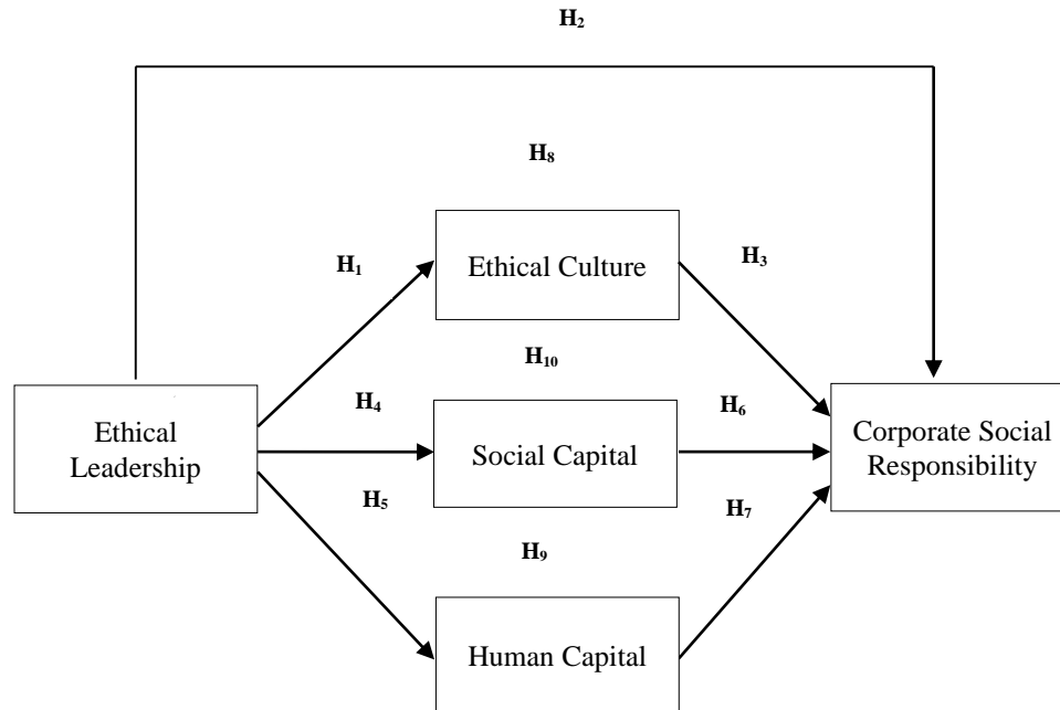
Figure 1: Proposed Model for the Study
