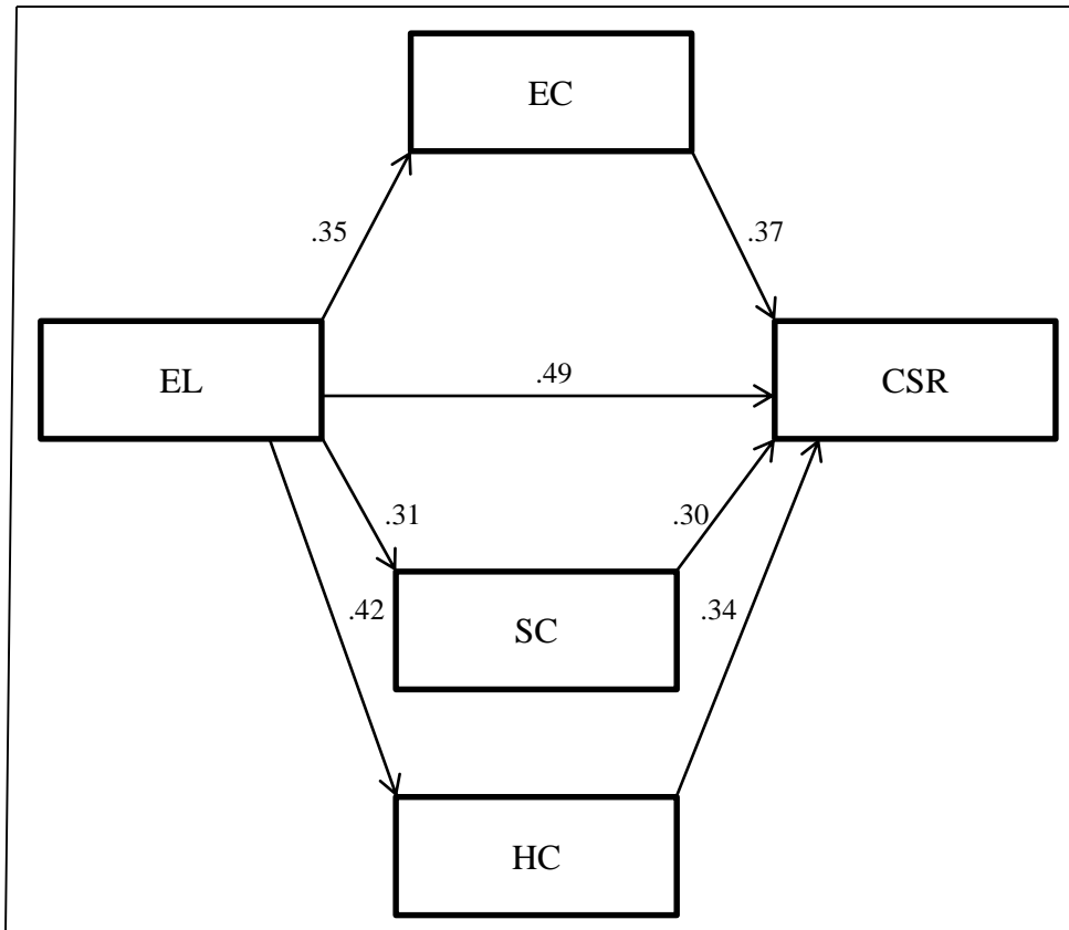
Figure 2: Path Diagram of Regression Analysis
