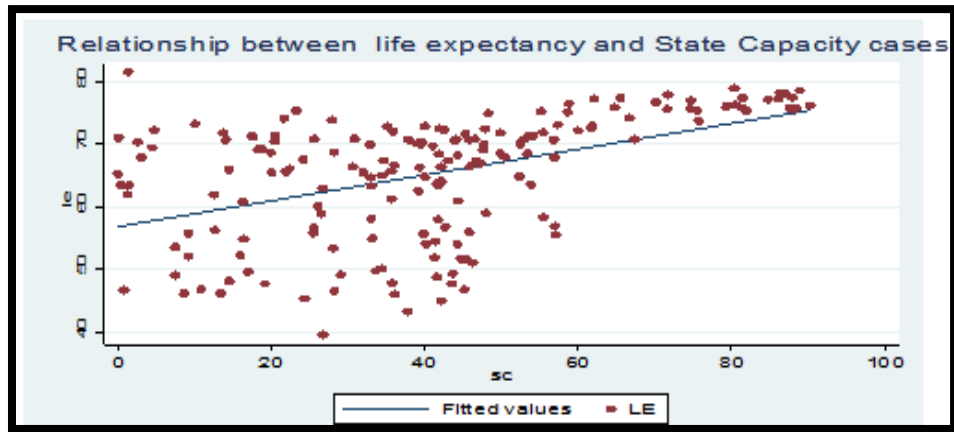
Figure 2: Graphical Analysis between State Capacity and Life Expectancy
