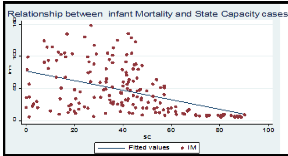
Figure 3: Graphical Analysis between State Capacity and Infant Mortality
