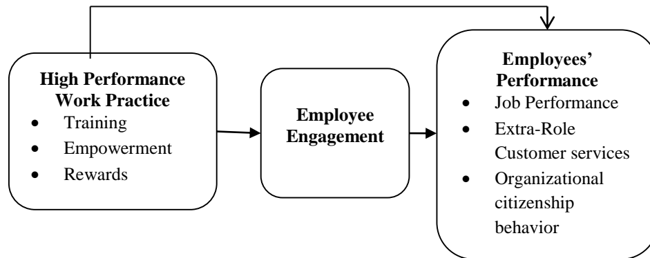
Fig. 1: Research Model
