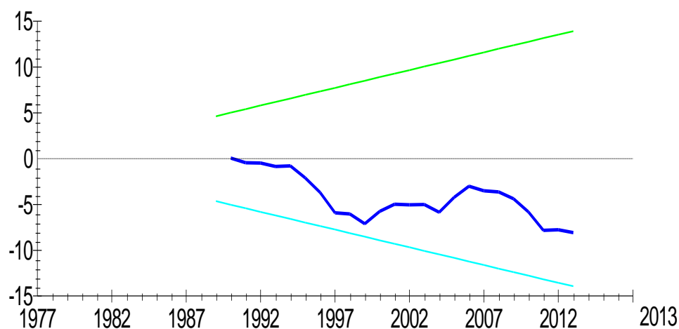
Figure 1: Stability Test for the Model-I [INV (IRD, INF, ER, MS, OPEN, GDPGR)]
