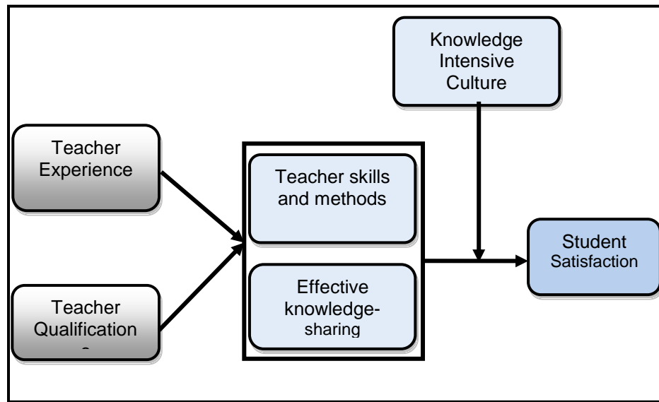
Figure 1: Theoretical Model
