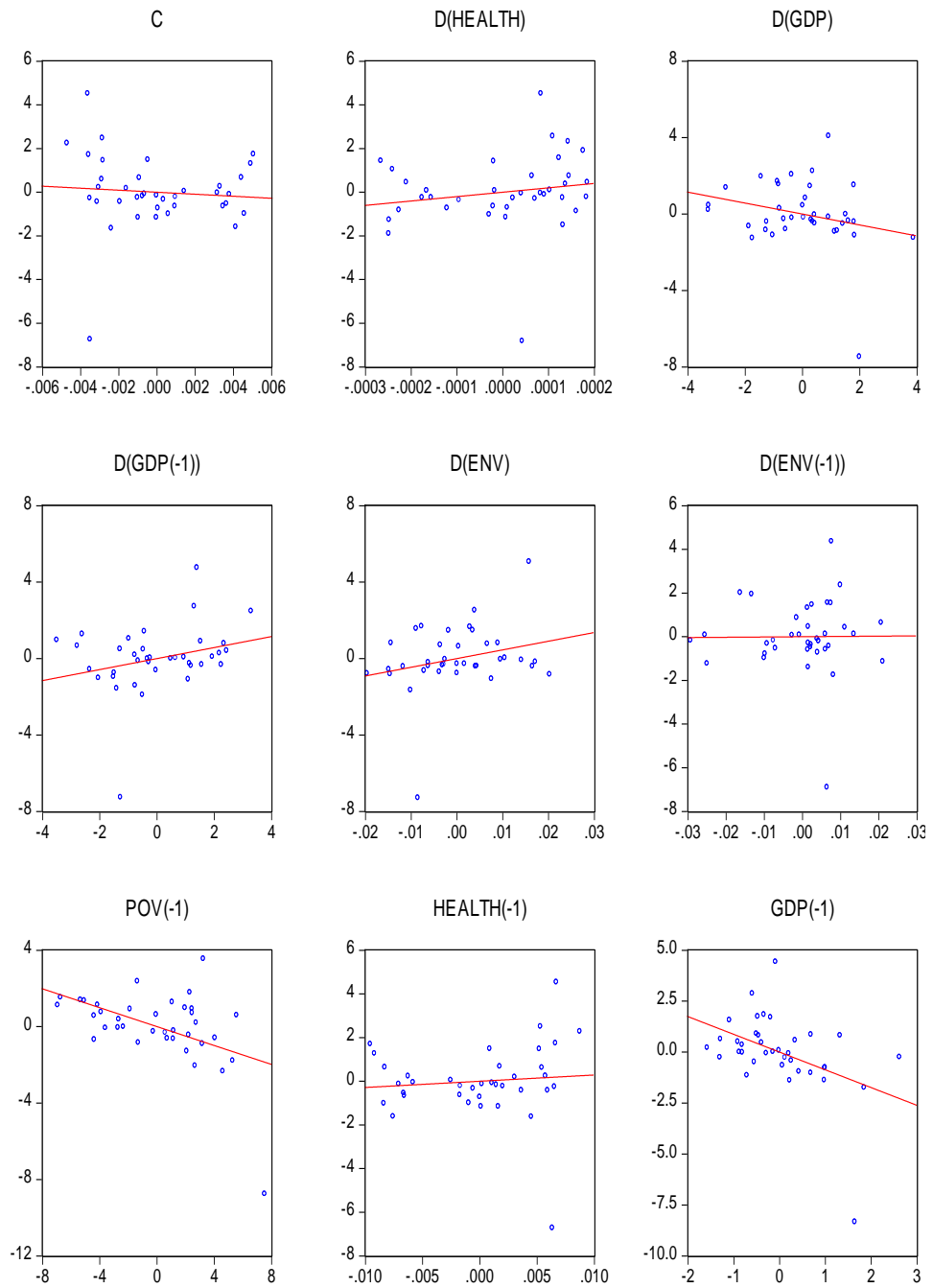
Figure 5: Leverage Plots
