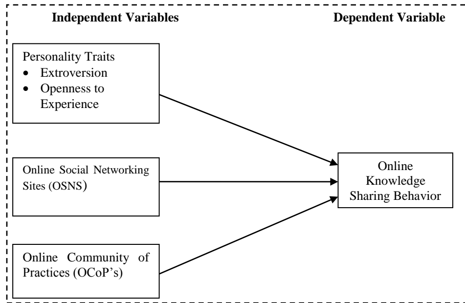
Figure 1: Theoretical Framework
