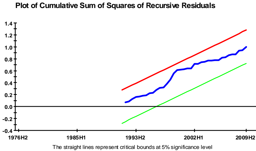
Figure 4: Plot of Z in Z-LTB model, residuals, CUSUM and CUSUMSQ
