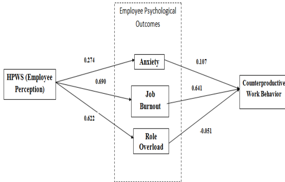
Figure 3: Structural Model with Regression Weights
