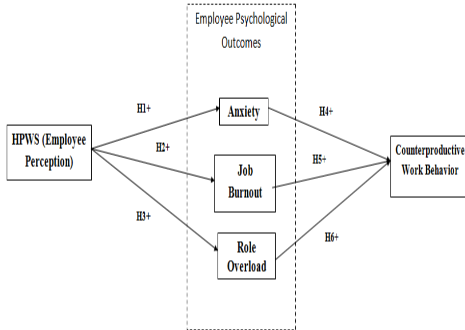
Figure1: Theoretical Model
