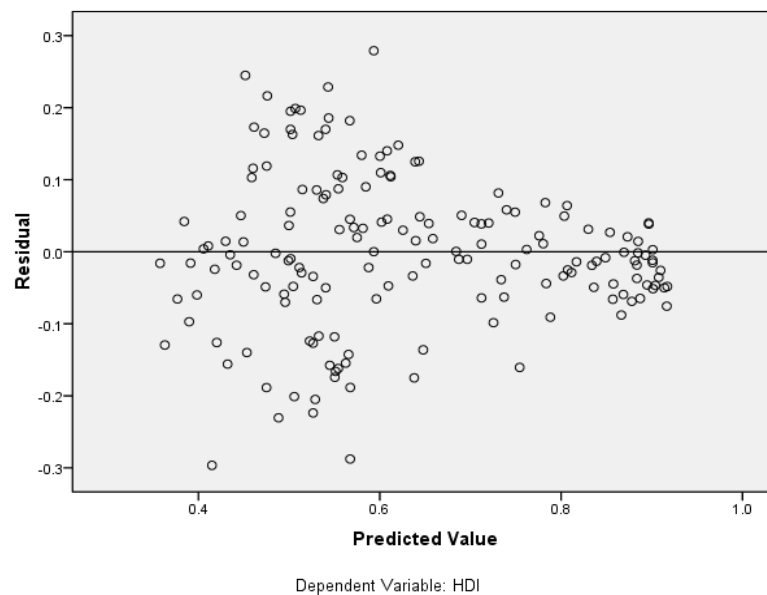
Figure 4: Residual by Predicted value Plot
