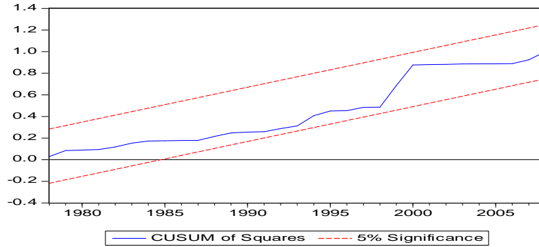
Figure 2: CUSUMsq Test
