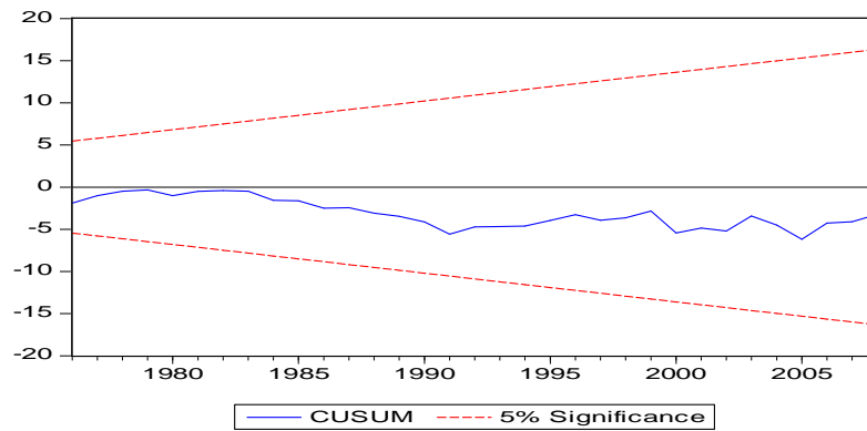
Figure 1: CUSUM Test
