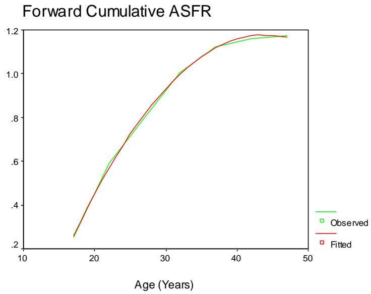
Figure 3: The graph of observed and fitted model of forward cumulative age specific fertility rates.
