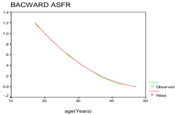
Figure 4: The graph of observed and fitted model of backward cumulative age-specific fertility rates.
