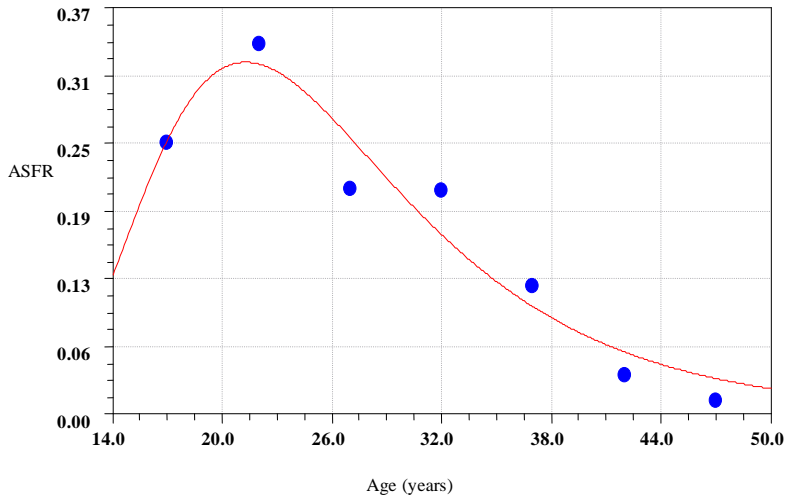
Figure 2: The graph of observed and fitted model of age-specific fertility rates.
