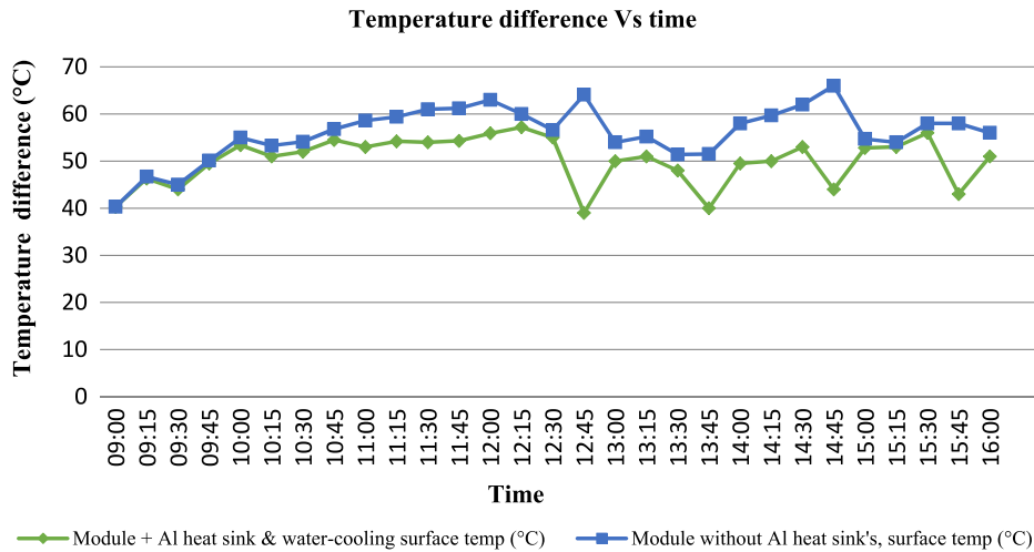
Fig. 11. A plot of module + Al heat sink & water-cooling and the module without Al heat sink's surface temperatures (°C) Vs time.
