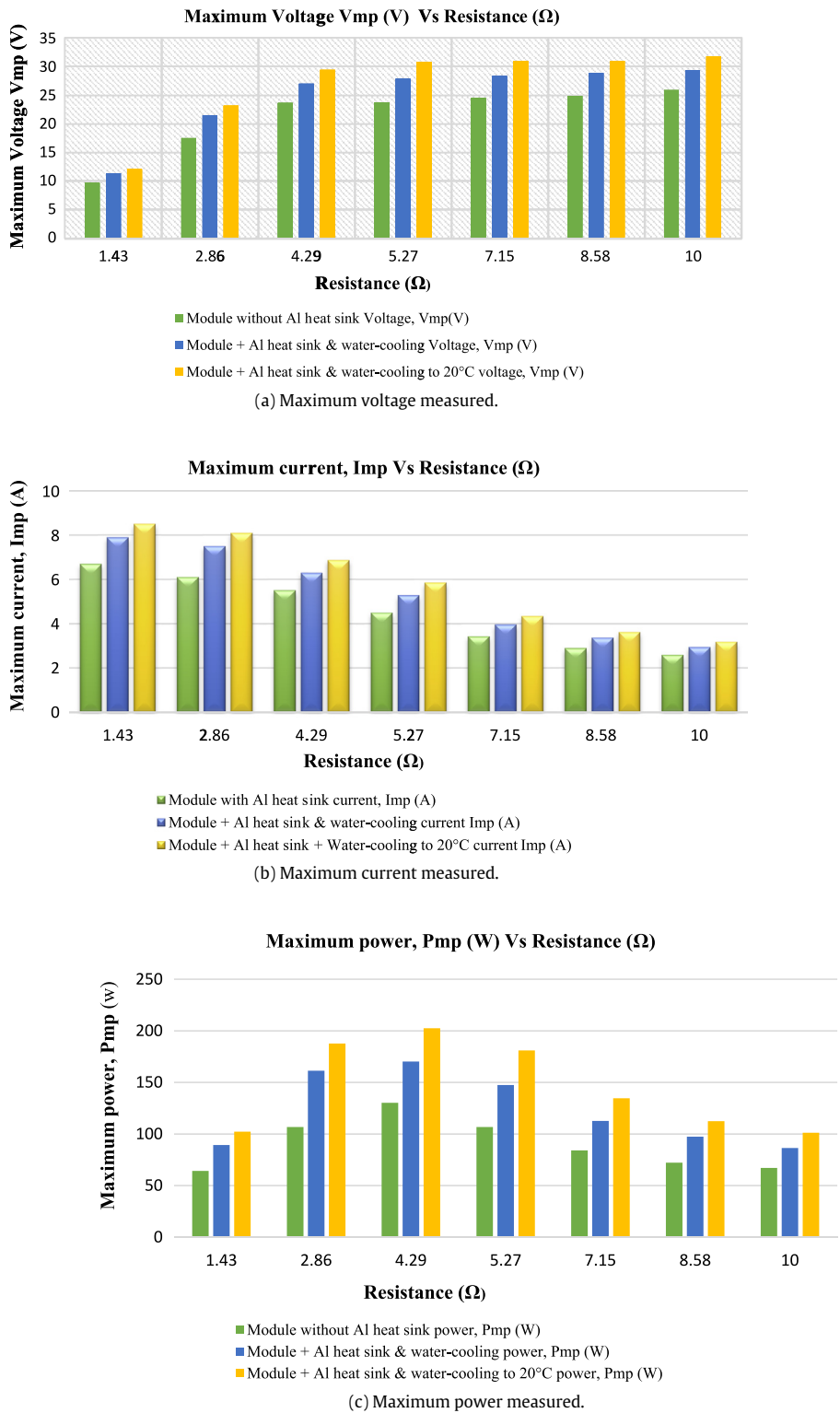
Fig. 13. (a) maximum voltage Vs load (b) maximum current Vs load (c) maximum power Vs load.
